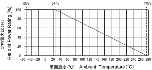
Power Derating Curve
