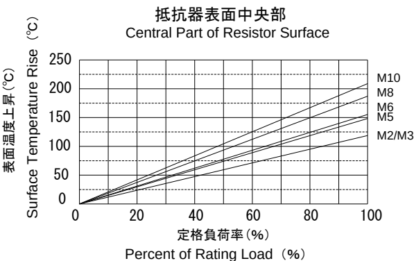
Surface Temperature Rising Curve
