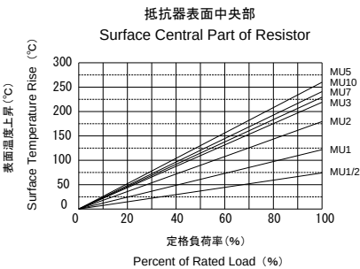
Surface Temperature Rising Curve
